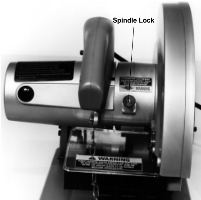
Figure 8 – Removing Saw Blade
