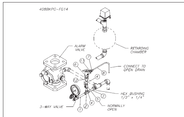
Figure 14—Open Retard Drain. UL Listed.
