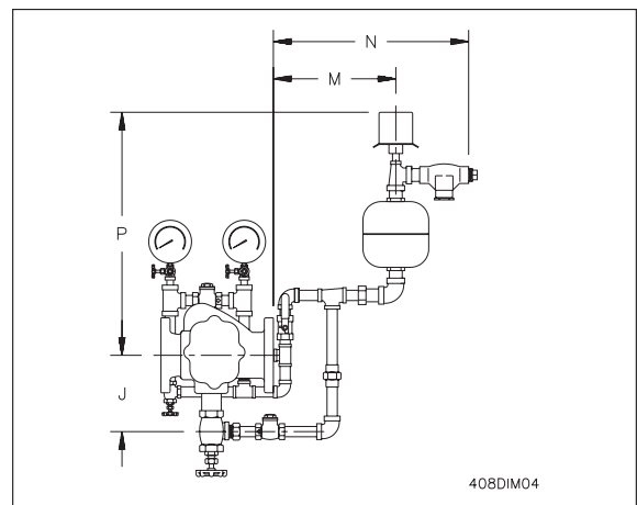
Variable Pressure, Horizontal, Closed Drain Trim Front Elevation
