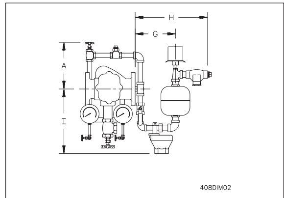
Variable Pressure, Horizontal Trim Front Elevation
