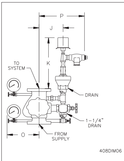
Constant Pressure, Vertical Trim Front Elevation
