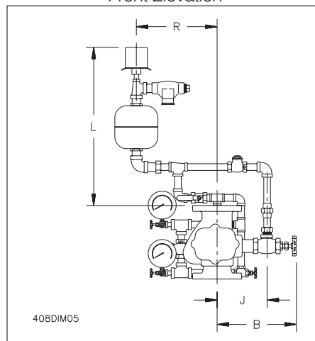
Variable Pressure, Vertical, Closed Drain Trim Front Elevation
