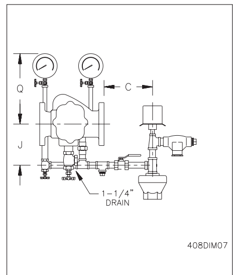
Constant Pressure, Horizontal Trim Front Elevation
