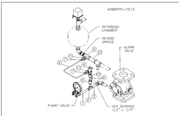
Figure 13—Closed Retard Drain. UL Listed.
