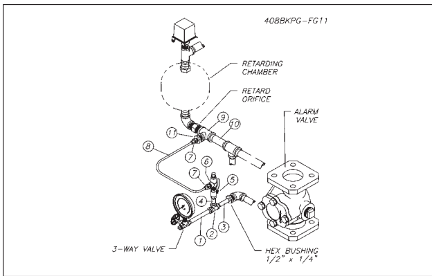
Figure 11—Closed Retard Drain. FM Approved
