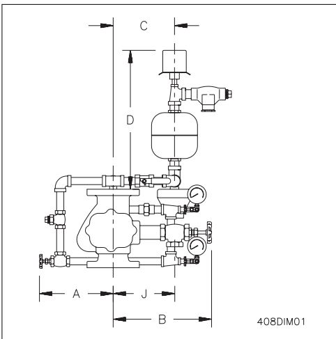
Variable Pressure, Vertical Trim Front Elevation
