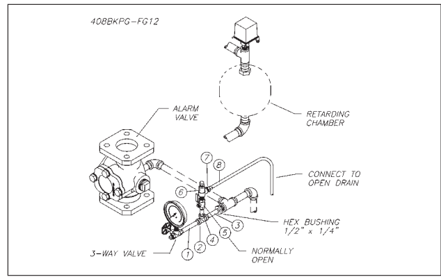
Figure 12—Open Retard Drain. FM Approved
