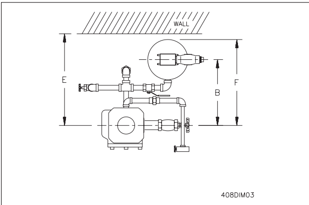
Variable Pressure, Vertical Trim Top View
